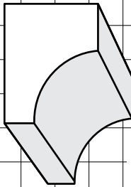
WM95 11/16" X 7/8"
