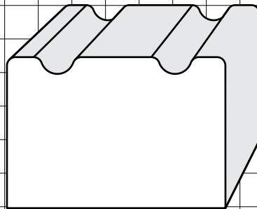
MK0030 1-1/8" X 1-5/8"
